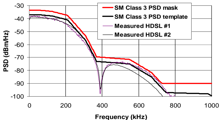
Fig. 4. Spectrum management class 3 (SM3) PSD mask, PSD template, and a couple of measured HDSL transmit PSDs.
