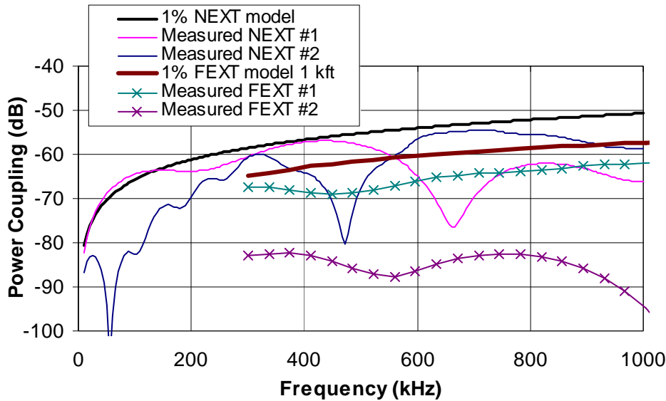
Fig. 2. 1% worst-case single crosstalk disturber crosstalk power coupling models and measurements of pair-to-pair NEXT and FEXT. FEXT is on a 1 kft 24 gauge loop.
