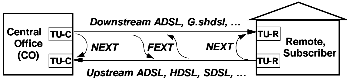
Fig. 1. NEXT and FEXT.
