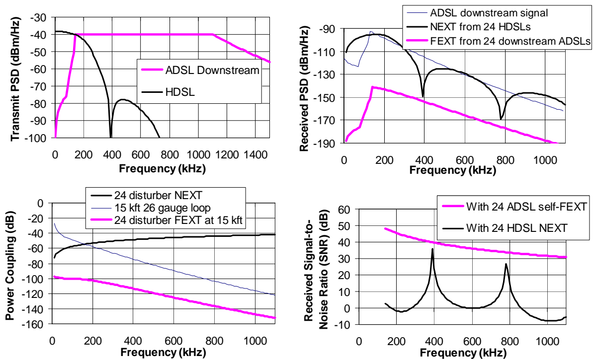
Fig. 3. Downstream ADSL performance with self-FEXT from 24 other ADSL crosstalk disturbers, and with 24 HDSL NEXT disturbers on a 15 kft 26 gauge loop.
